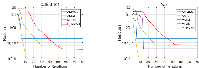
Fig. 7. Average empirical convergence curves of different algorithms on Caltech101 and Yale databases.
